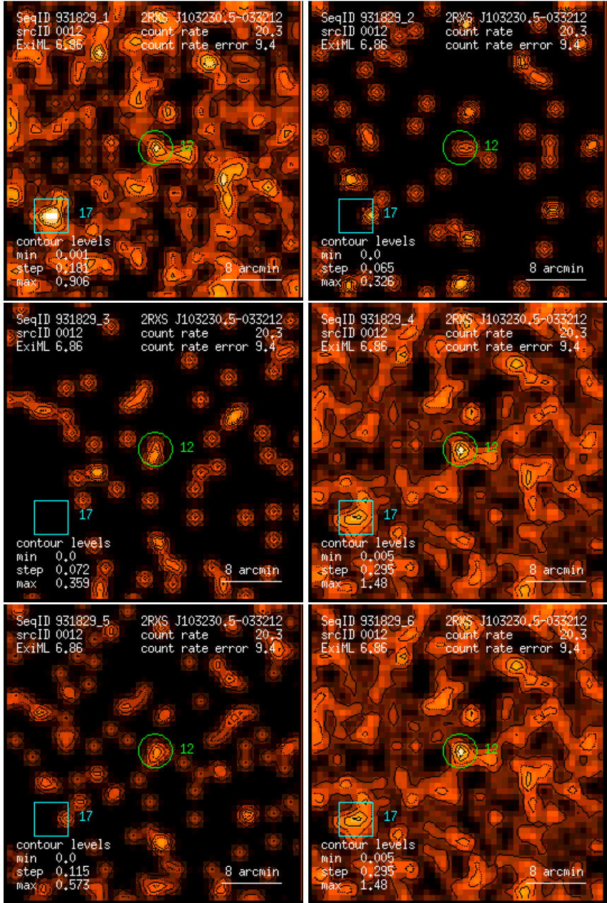
Figure 12: RASS 931829: detection 0012: band rate images, Gaussian filter: (1) PSPC channels 11 – 41, (2) 52 – 90, (3) 91 – 201, (4) 11 – 235, (5) 52 – 201, (6) 11 – 201. Broad band rates in counts/ks. Band rate contour levels in counts/ks/arcmin 2 .
