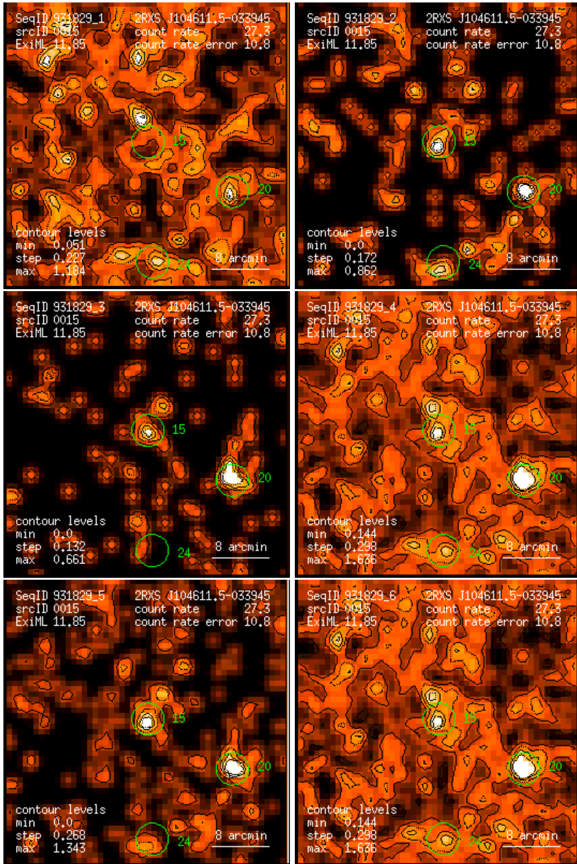
Figure 15: RASS 931829: detection 0015: band rate images, Gaussian filter: (1) PSPC channels 11 – 41, (2) 52 – 90, (3) 91 – 201, (4) 11 – 235, (5) 52 – 201, (6) 11 – 201. Broad band rates in counts/ks. Band rate contour levels in counts/ks/arcmin 2 .
