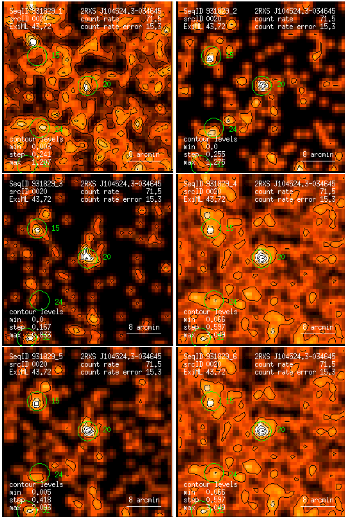
Figure 20: RASS 931829: detection 0020: band rate images, Gaussian filter: (1) PSPC channels 11 – 41, (2) 52 – 90, (3) 91 – 201, (4) 11 – 235, (5) 52 – 201, (6) 11 – 201. Broad band rates in counts/ks. Band rate contour levels in counts/ks/arcmin 2 .
