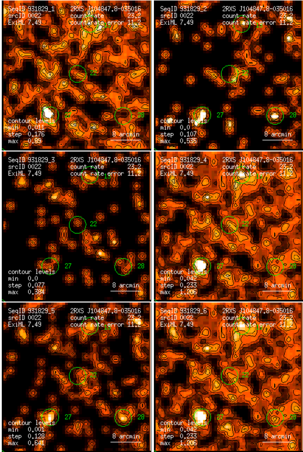
Figure 22: RASS 931829: detection 0022: band rate images, Gaussian filter: (1) PSPC channels 11 – 41, (2) 52 – 90, (3) 91 – 201, (4) 11 – 235, (5) 52 – 201, (6) 11 – 201. Broad band rates in counts/ks. Band rate contour levels in counts/ks/arcmin 2 .
