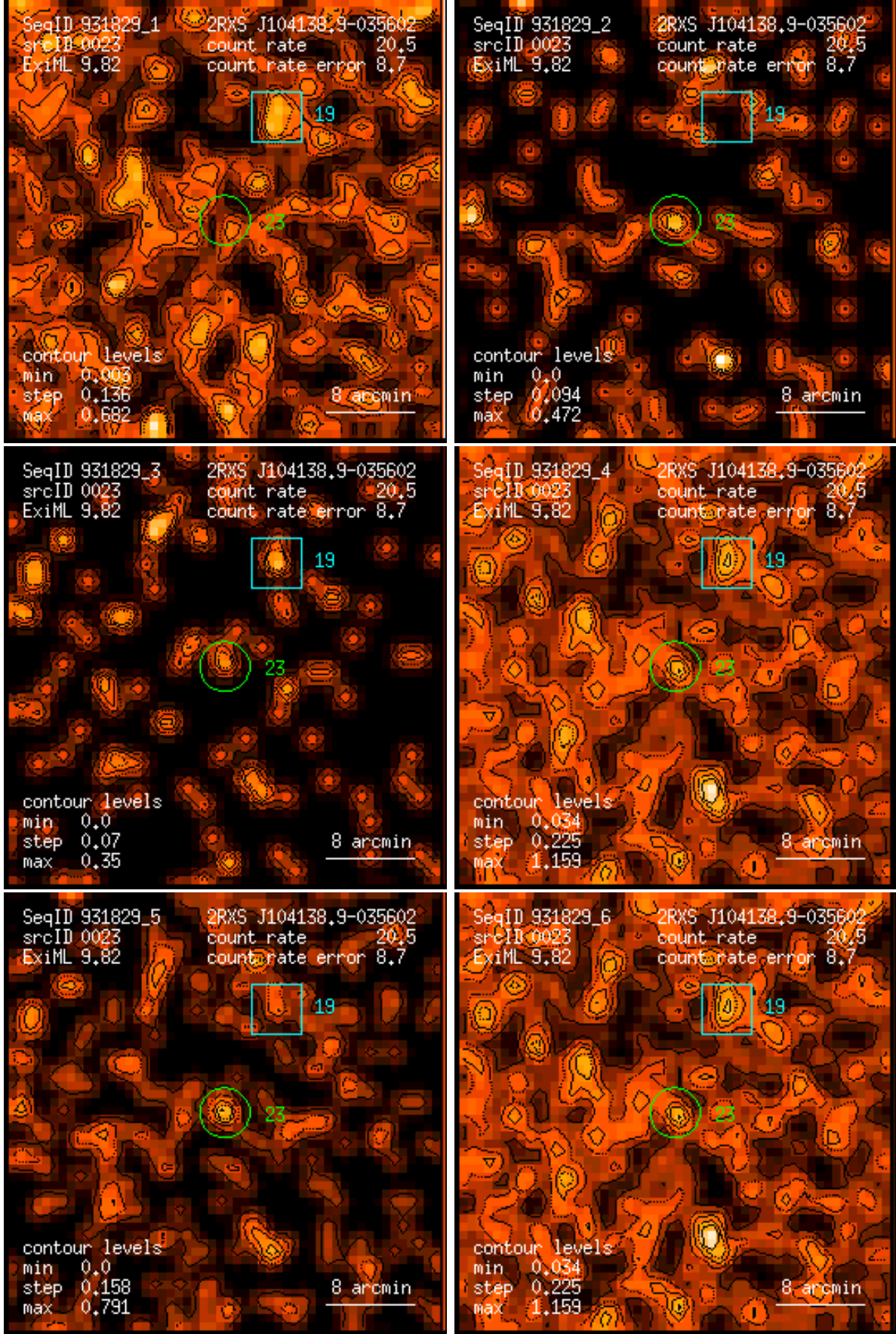
Figure 23: RASS 931829: detection 0023: band rate images, Gaussian filter: (1) PSPC channels 11 – 41, (2) 52 – 90, (3) 91 – 201, (4) 11 – 235, (5) 52 – 201, (6) 11 – 201. Broad band rates in counts/ks. Band rate contour levels in counts/ks/arcmin 2 .
