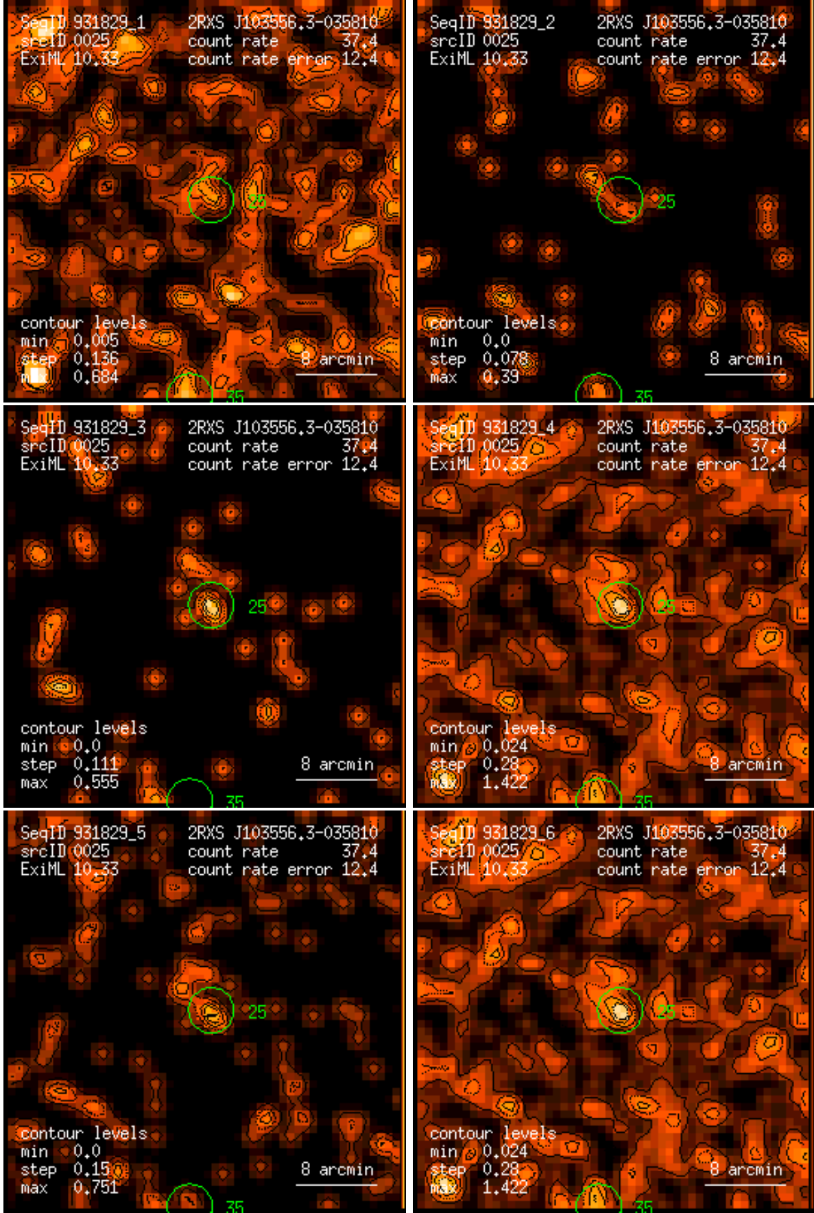
Figure 25: RASS 931829: detection 0025: band rate images, Gaussian filter: (1) PSPC channels 11 – 41, (2) 52 – 90, (3) 91 – 201, (4) 11 – 235, (5) 52 – 201, (6) 11 – 201. Broad band rates in counts/ks. Band rate contour levels in counts/ks/arcmin 2 .
