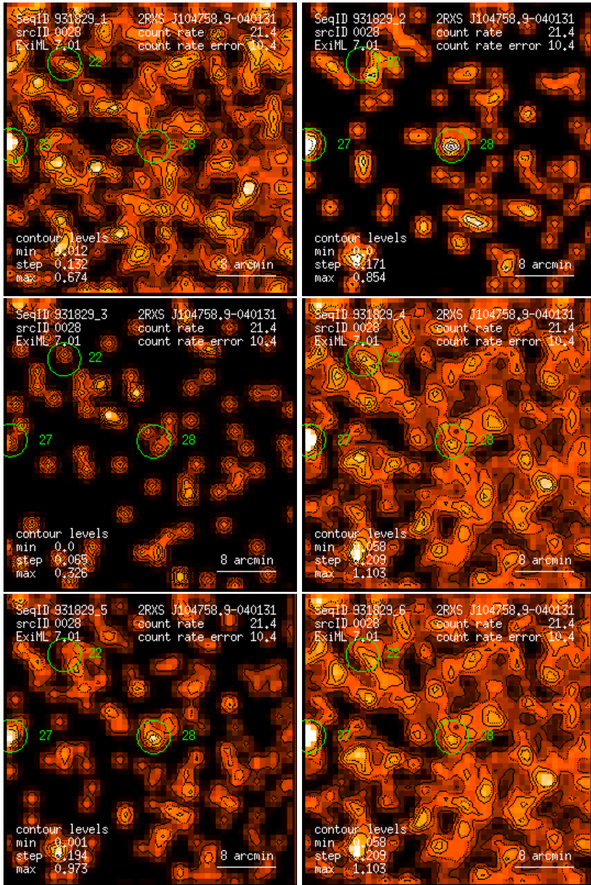
Figure 28: RASS 931829: detection 0028: band rate images, Gaussian filter: (1) PSPC channels 11 – 41, (2) 52 – 90, (3) 91 – 201, (4) 11 – 235, (5) 52 – 201, (6) 11 – 201. Broad band rates in counts/ks. Band rate contour levels in counts/ks/arcmin 2 .
