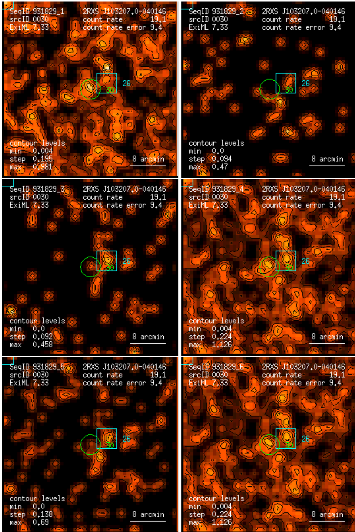
Figure 30: RASS 931829: detection 0030: band rate images, Gaussian filter: (1) PSPC channels 11 – 41, (2) 52 – 90, (3) 91 – 201, (4) 11 – 235, (5) 52 – 201, (6) 11 – 201. Broad band rates in counts/ks. Band rate contour levels in counts/ks/arcmin 2 .
