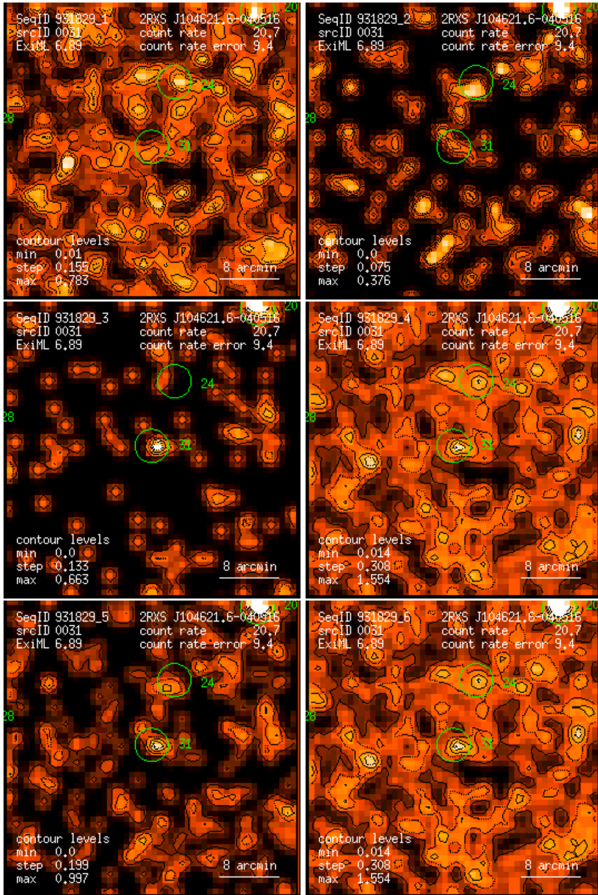
Figure 31: RASS 931829: detection 0031: band rate images, Gaussian filter: (1) PSPC channels 11 – 41, (2) 52 – 90, (3) 91 – 201, (4) 11 – 235, (5) 52 – 201, (6) 11 – 201. Broad band rates in counts/ks. Band rate contour levels in counts/ks/arcmin 2 .
