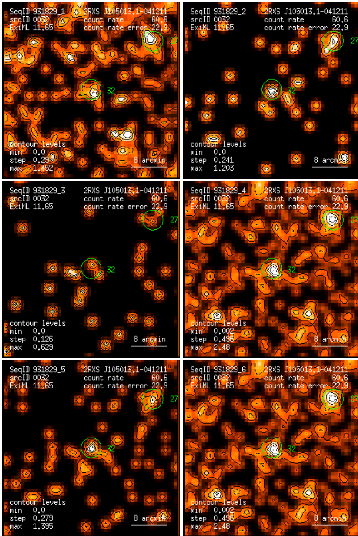
Figure 32: RASS 931829: detection 0032: band rate images, Gaussian filter: (1) PSPC channels 11 – 41, (2) 52 – 90, (3) 91 – 201, (4) 11 – 235, (5) 52 – 201, (6) 11 – 201. Broad band rates in counts/ks. Band rate contour levels in counts/ks/arcmin 2 .
