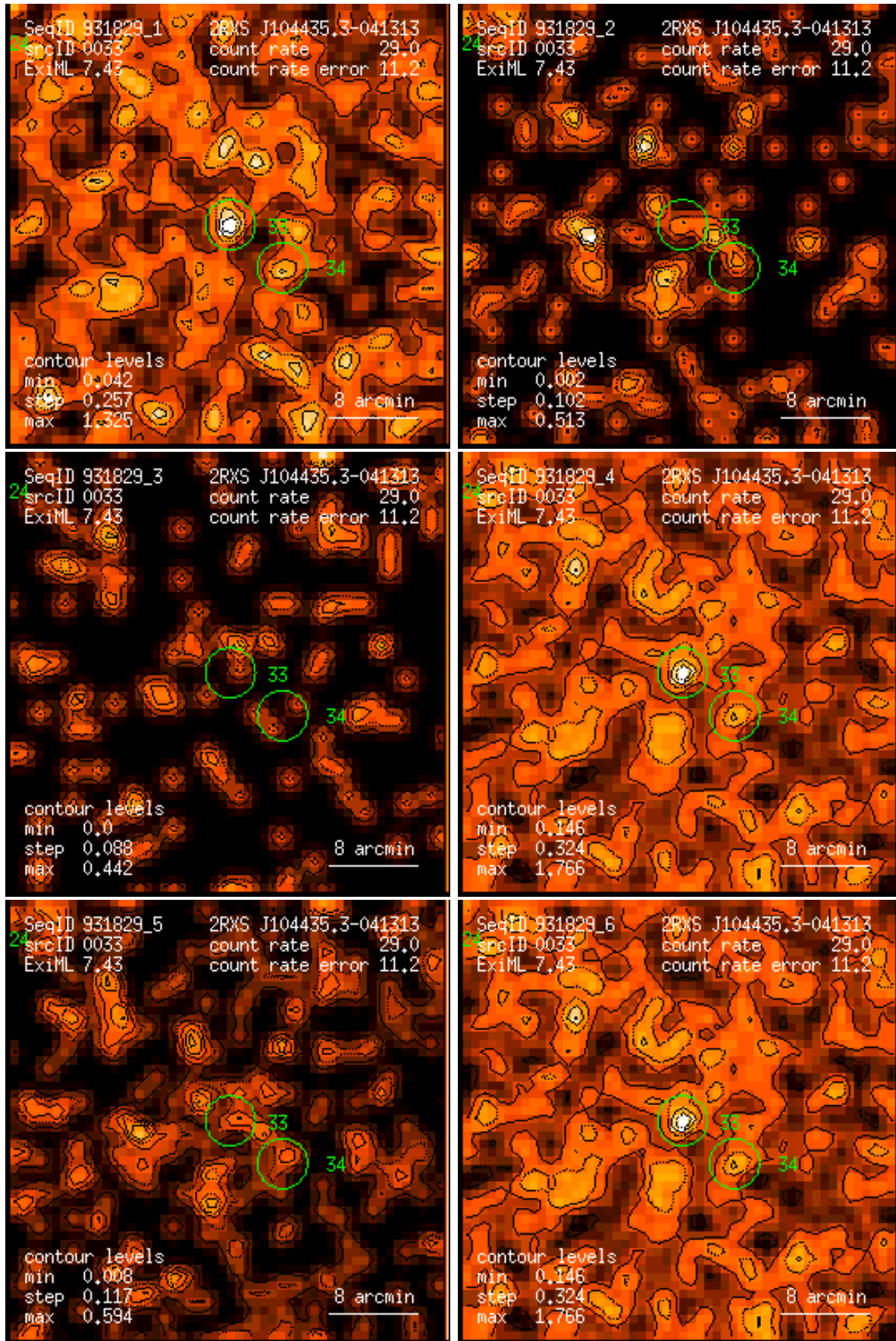
Figure 33: RASS 931829: detection 0033: band rate images, Gaussian filter: (1) PSPC channels 11 – 41, (2) 52 – 90, (3) 91 – 201, (4) 11 – 235, (5) 52 – 201, (6) 11 – 201. Broad band rates in counts/ks. Band rate contour levels in counts/ks/arcmin 2 .
