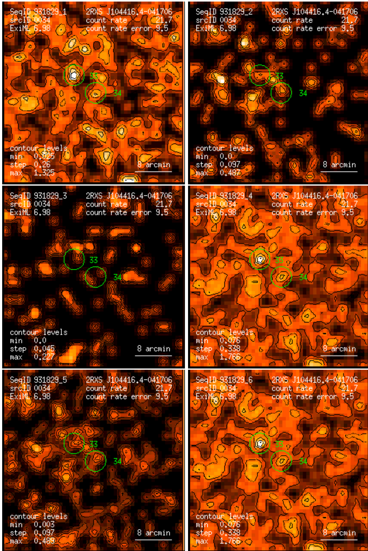
Figure 34: RASS 931829: detection 0034: band rate images, Gaussian filter: (1) PSPC channels 11 – 41, (2) 52 – 90, (3) 91 – 201, (4) 11 – 235, (5) 52 – 201, (6) 11 – 201. Broad band rates in counts/ks. Band rate contour levels in counts/ks/arcmin 2 .
