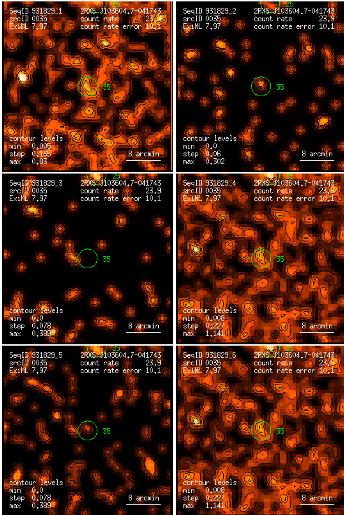
Figure 35: RASS 931829: detection 0035: band rate images, Gaussian filter: (1) PSPC channels 11 – 41, (2) 52 – 90, (3) 91 – 201, (4) 11 – 235, (5) 52 – 201, (6) 11 – 201. Broad band rates in counts/ks. Band rate contour levels in counts/ks/arcmin 2 .
