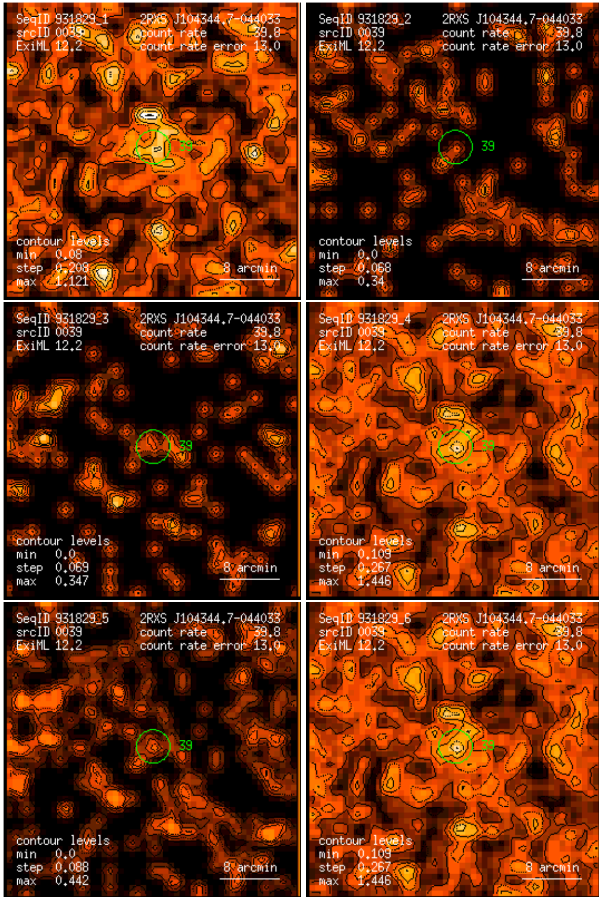
Figure 39: RASS 931829: detection 0039: band rate images, Gaussian filter: (1) PSPC channels 11 – 41, (2) 52 – 90, (3) 91 – 201, (4) 11 – 235, (5) 52 – 201, (6) 11 – 201. Broad band rates in counts/ks. Band rate contour levels in counts/ks/arcmin 2 .
