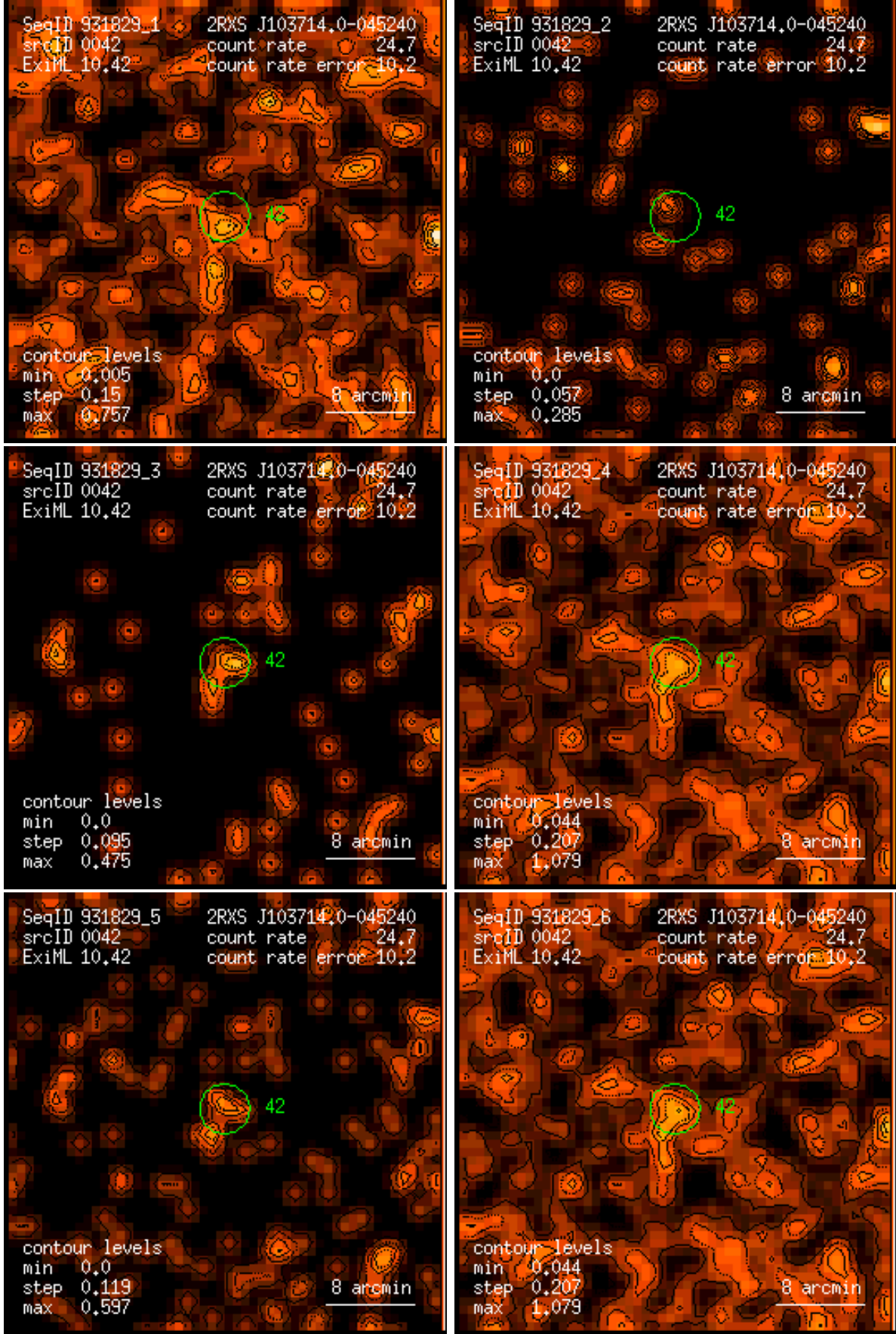
Figure 42: RASS 931829: detection 0042: band rate images, Gaussian filter: (1) PSPC channels 11 – 41, (2) 52 – 90, (3) 91 – 201, (4) 11 – 235, (5) 52 – 201, (6) 11 – 201. Broad band rates in counts/ks. Band rate contour levels in counts/ks/arcmin 2 .
