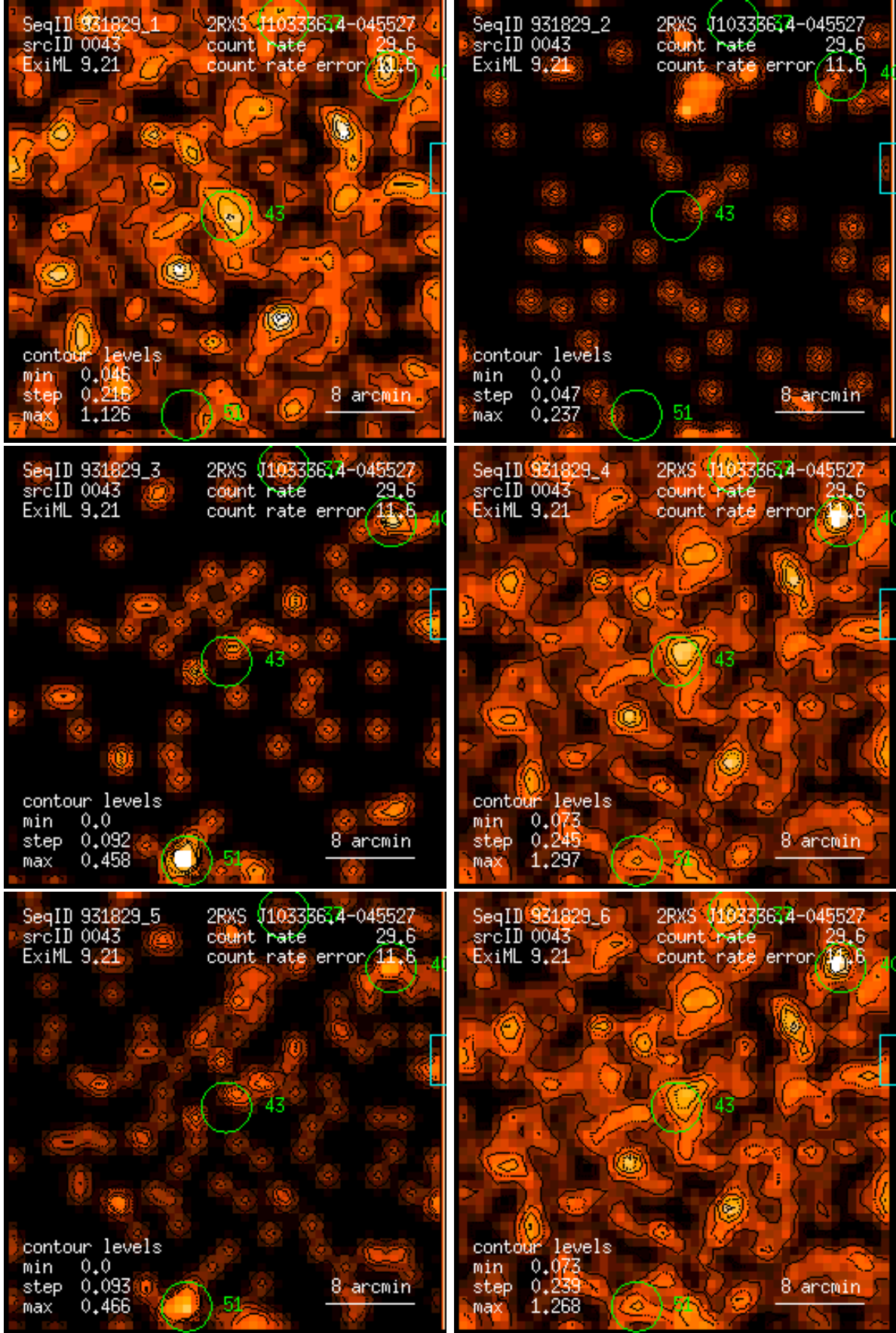
Figure 43: RASS 931829: detection 0043: band rate images, Gaussian filter: (1) PSPC channels 11 – 41, (2) 52 – 90, (3) 91 – 201, (4) 11 – 235, (5) 52 – 201, (6) 11 – 201. Broad band rates in counts/ks. Band rate contour levels in counts/ks/arcmin 2 .
