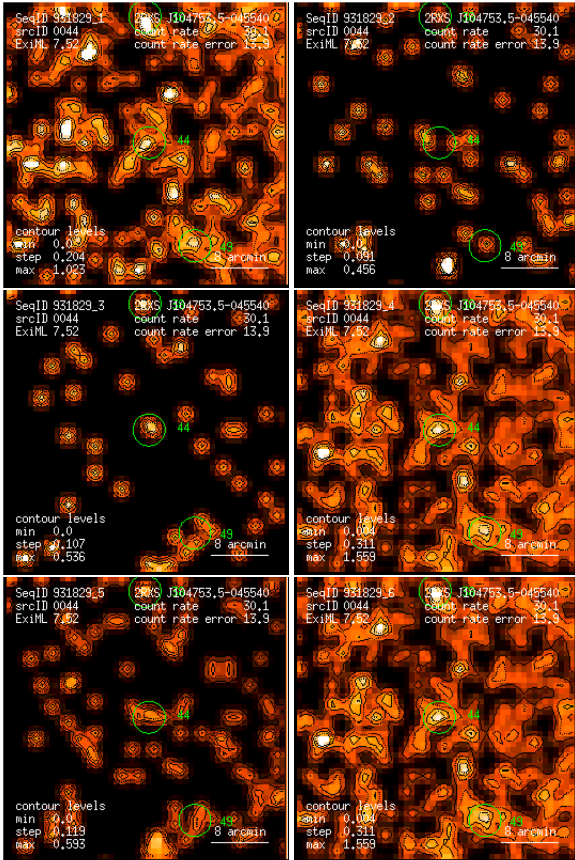
Figure 44: RASS 931829: detection 0044: band rate images, Gaussian filter: (1) PSPC channels 11 – 41, (2) 52 – 90, (3) 91 – 201, (4) 11 – 235, (5) 52 – 201, (6) 11 – 201. Broad band rates in counts/ks. Band rate contour levels in counts/ks/arcmin 2 .
