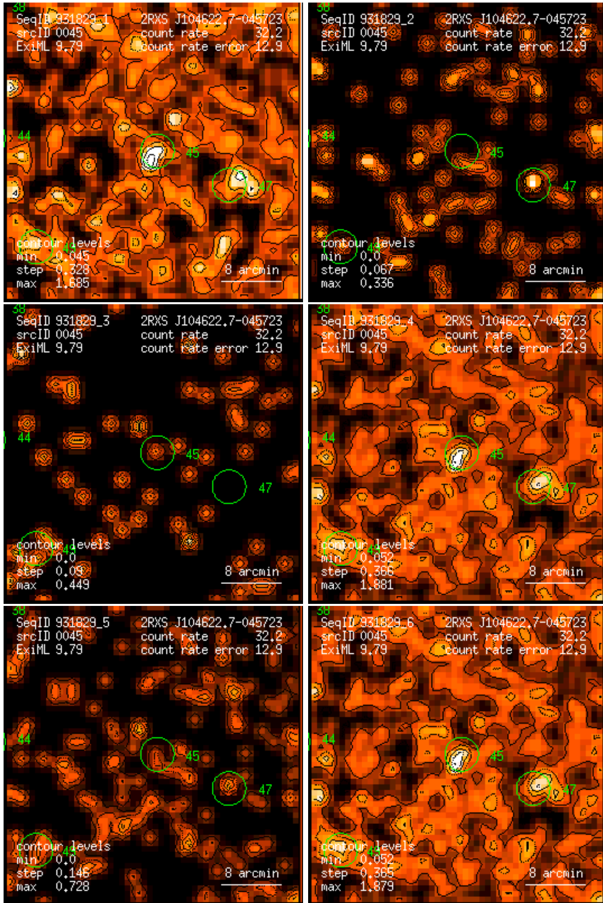
Figure 45: RASS 931829: detection 0045: band rate images, Gaussian filter: (1) PSPC channels 11 – 41, (2) 52 – 90, (3) 91 – 201, (4) 11 – 235, (5) 52 – 201, (6) 11 – 201. Broad band rates in counts/ks. Band rate contour levels in counts/ks/arcmin 2 .
