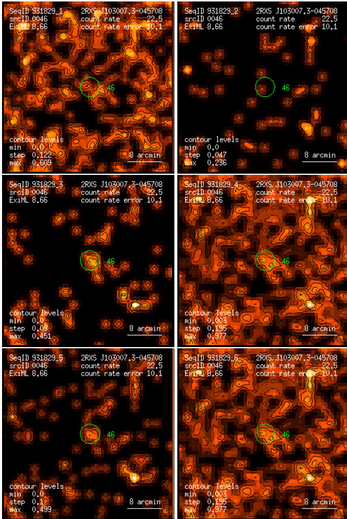
Figure 46: RASS 931829: detection 0046: band rate images, Gaussian filter: (1) PSPC channels 11 – 41, (2) 52 – 90, (3) 91 – 201, (4) 11 – 235, (5) 52 – 201, (6) 11 – 201. Broad band rates in counts/ks. Band rate contour levels in counts/ks/arcmin 2 .
