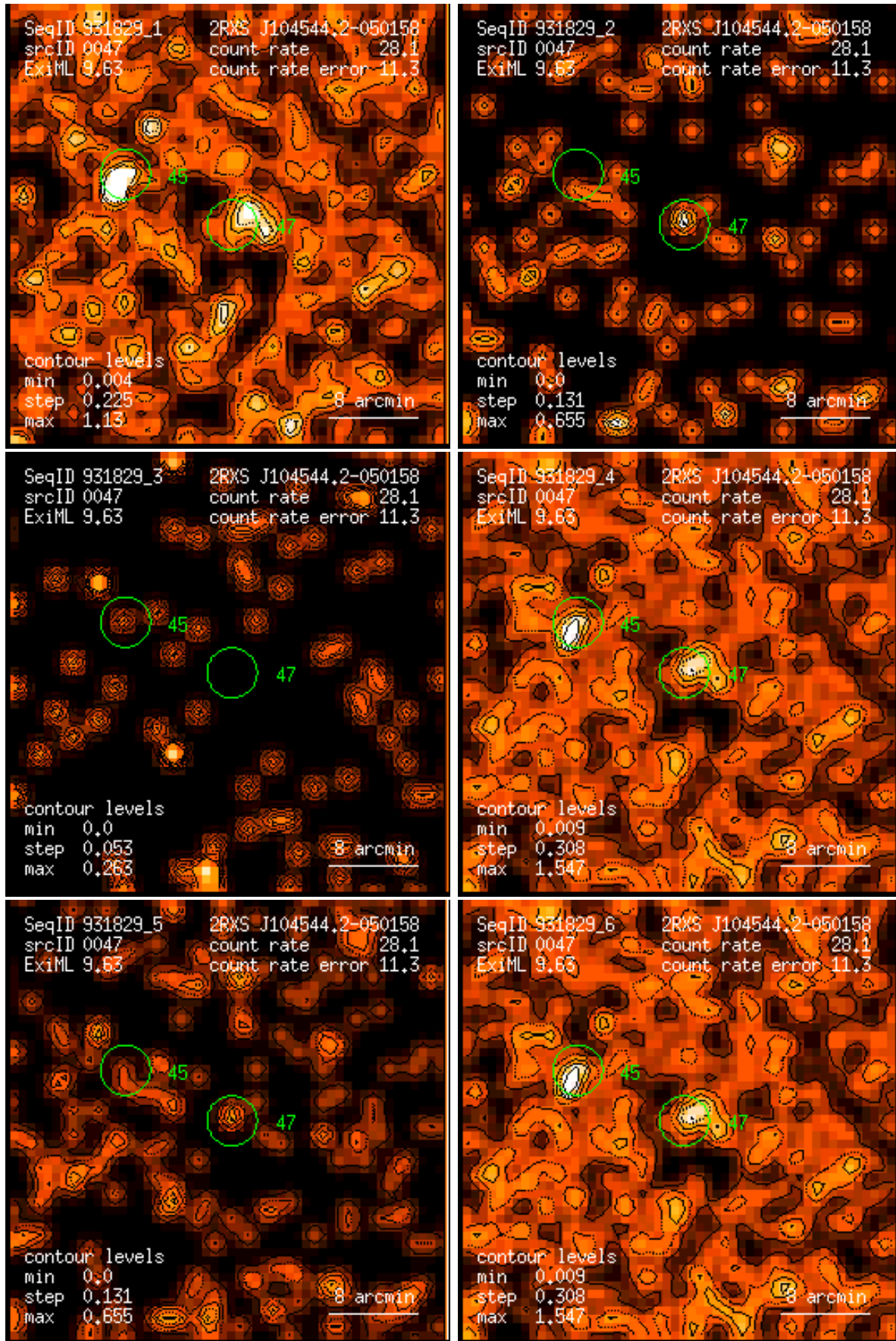
Figure 47: RASS 931829: detection 0047: band rate images, Gaussian filter: (1) PSPC channels 11 – 41, (2) 52 – 90, (3) 91 – 201, (4) 11 – 235, (5) 52 – 201, (6) 11 – 201. Broad band rates in counts/ks. Band rate contour levels in counts/ks/arcmin 2 .
