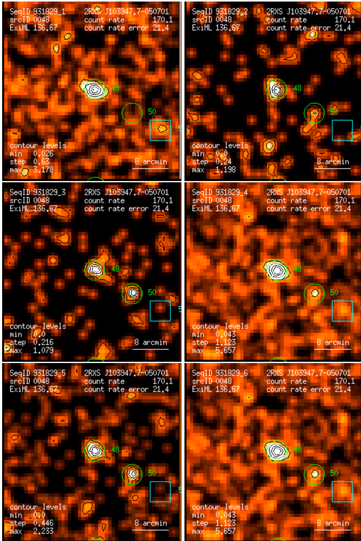
Figure 48: RASS 931829: detection 0048: band rate images, Gaussian filter: (1) PSPC channels 11 – 41, (2) 52 – 90, (3) 91 – 201, (4) 11 – 235, (5) 52 – 201, (6) 11 – 201. Broad band rates in counts/ks. Band rate contour levels in counts/ks/arcmin 2 .
