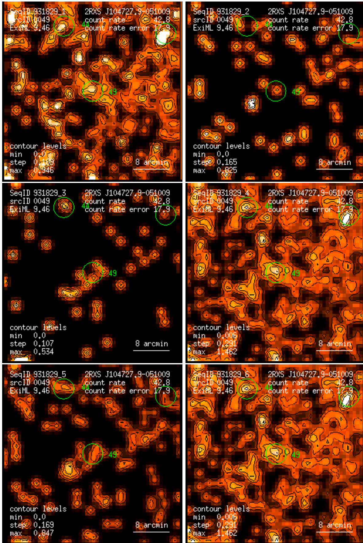
Figure 49: RASS 931829: detection 0049: band rate images, Gaussian filter: (1) PSPC channels 11 – 41, (2) 52 – 90, (3) 91 – 201, (4) 11 – 235, (5) 52 – 201, (6) 11 – 201. Broad band rates in counts/ks. Band rate contour levels in counts/ks/arcmin 2 .
