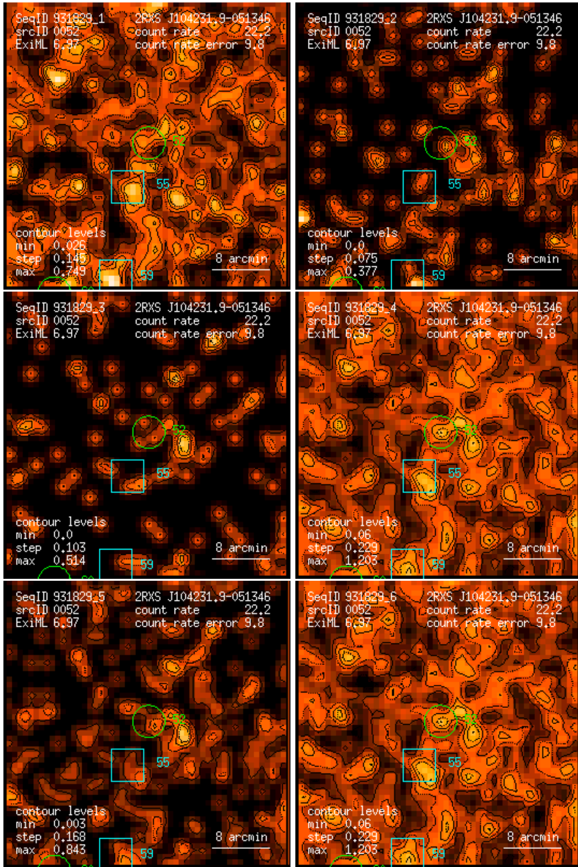
Figure 52: RASS 931829: detection 0052: band rate images, Gaussian filter: (1) PSPC channels 11 – 41, (2) 52 – 90, (3) 91 – 201, (4) 11 – 235, (5) 52 – 201, (6) 11 – 201. Broad band rates in counts/ks. Band rate contour levels in counts/ks/arcmin 2 .
