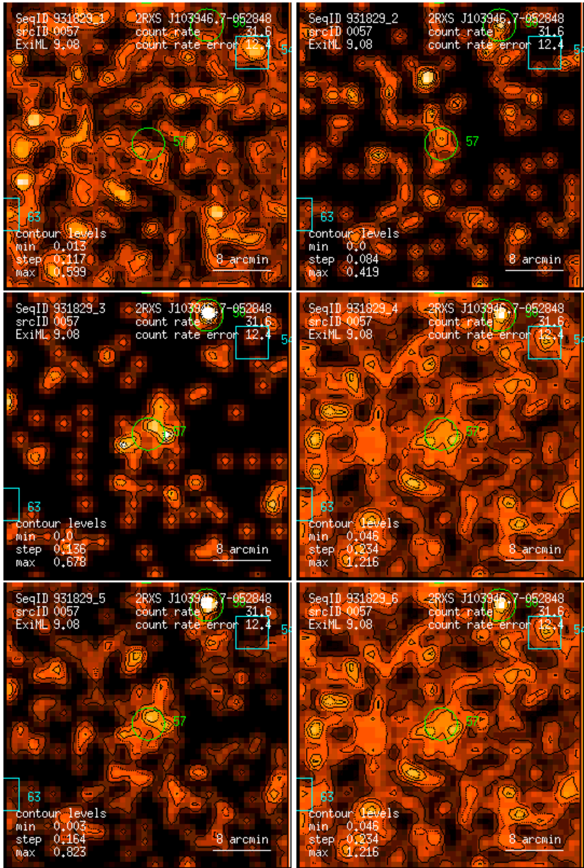
Figure 57: RASS 931829: detection 0057: band rate images, Gaussian filter: (1) PSPC channels 11 – 41, (2) 52 – 90, (3) 91 – 201, (4) 11 – 235, (5) 52 – 201, (6) 11 – 201. Broad band rates in counts/ks. Band rate contour levels in counts/ks/arcmin 2 .
