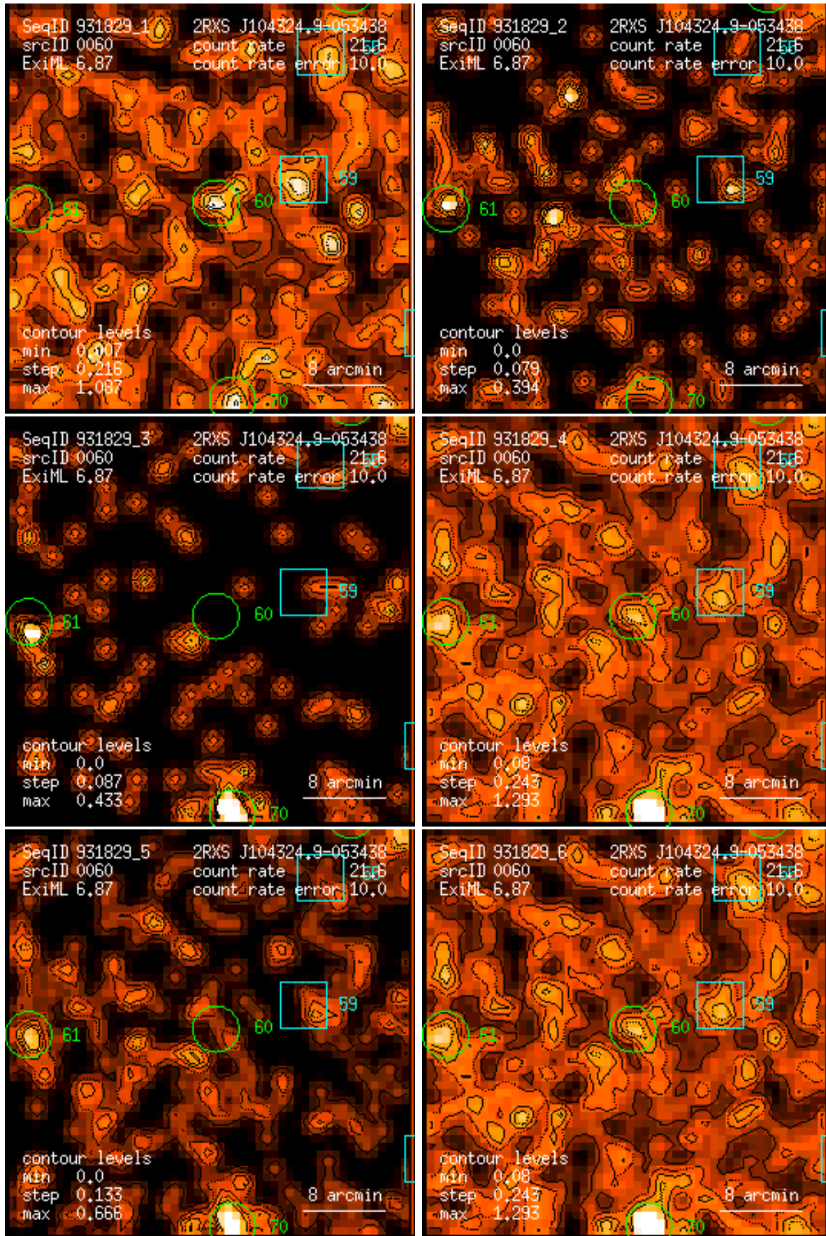
Figure 60: RASS 931829: detection 0060: band rate images, Gaussian filter: (1) PSPC channels 11 – 41, (2) 52 – 90, (3) 91 – 201, (4) 11 – 235, (5) 52 – 201, (6) 11 – 201. Broad band rates in counts/ks. Band rate contour levels in counts/ks/arcmin 2 .
