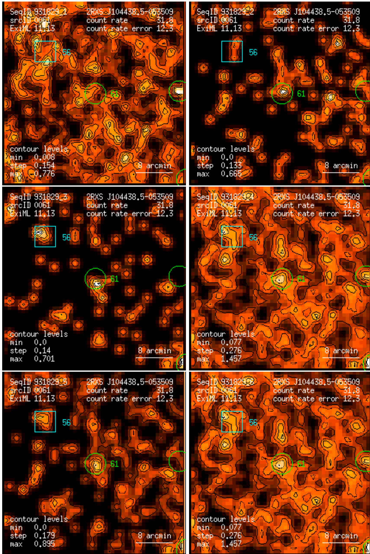
Figure 61: RASS 931829: detection 0061: band rate images, Gaussian filter: (1) PSPC channels 11 – 41, (2) 52 – 90, (3) 91 – 201, (4) 11 – 235, (5) 52 – 201, (6) 11 – 201. Broad band rates in counts/ks. Band rate contour levels in counts/ks/arcmin 2 .
