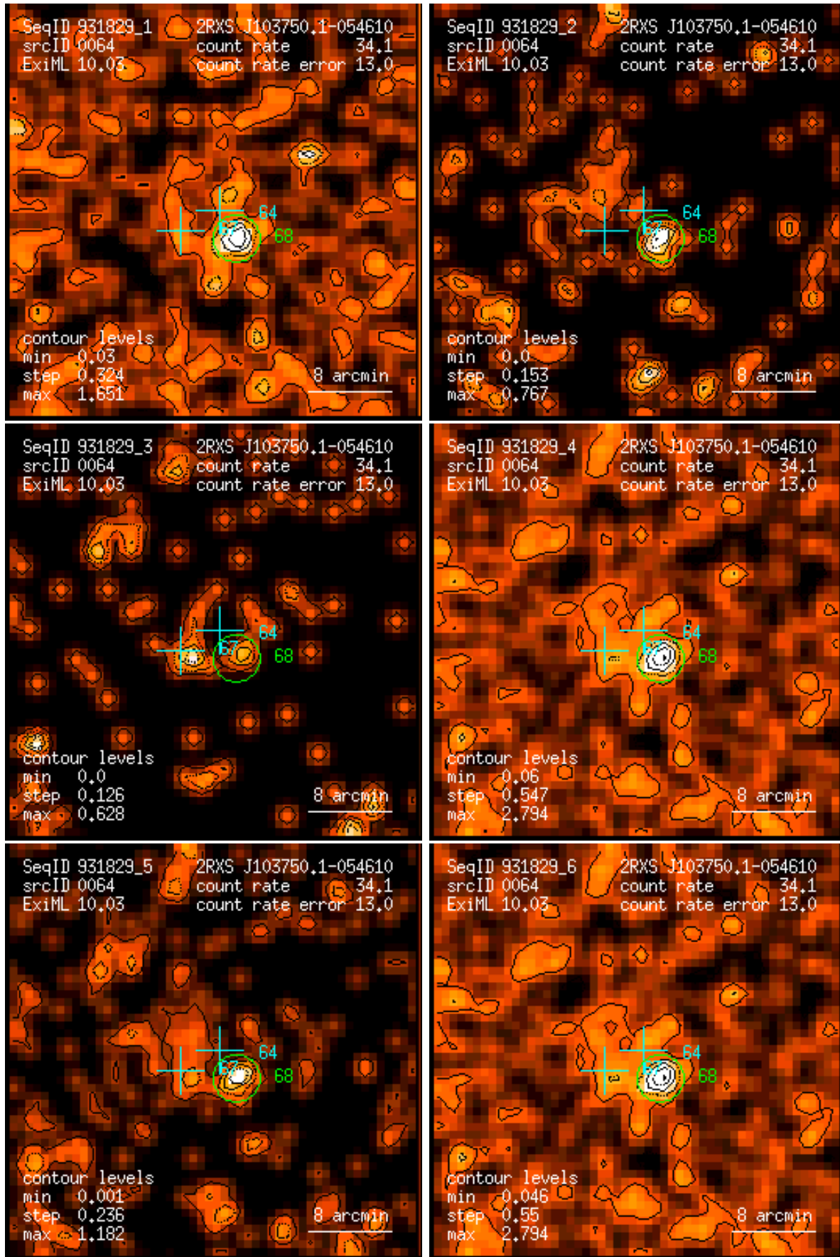
Figure 64: RASS 931829: detection 0064: band rate images, Gaussian filter: (1) PSPC channels 11 – 41, (2) 52 – 90, (3) 91 – 201, (4) 11 – 235, (5) 52 – 201, (6) 11 – 201. Broad band rates in counts/ks. Band rate contour levels in counts/ks/arcmin 2 .
