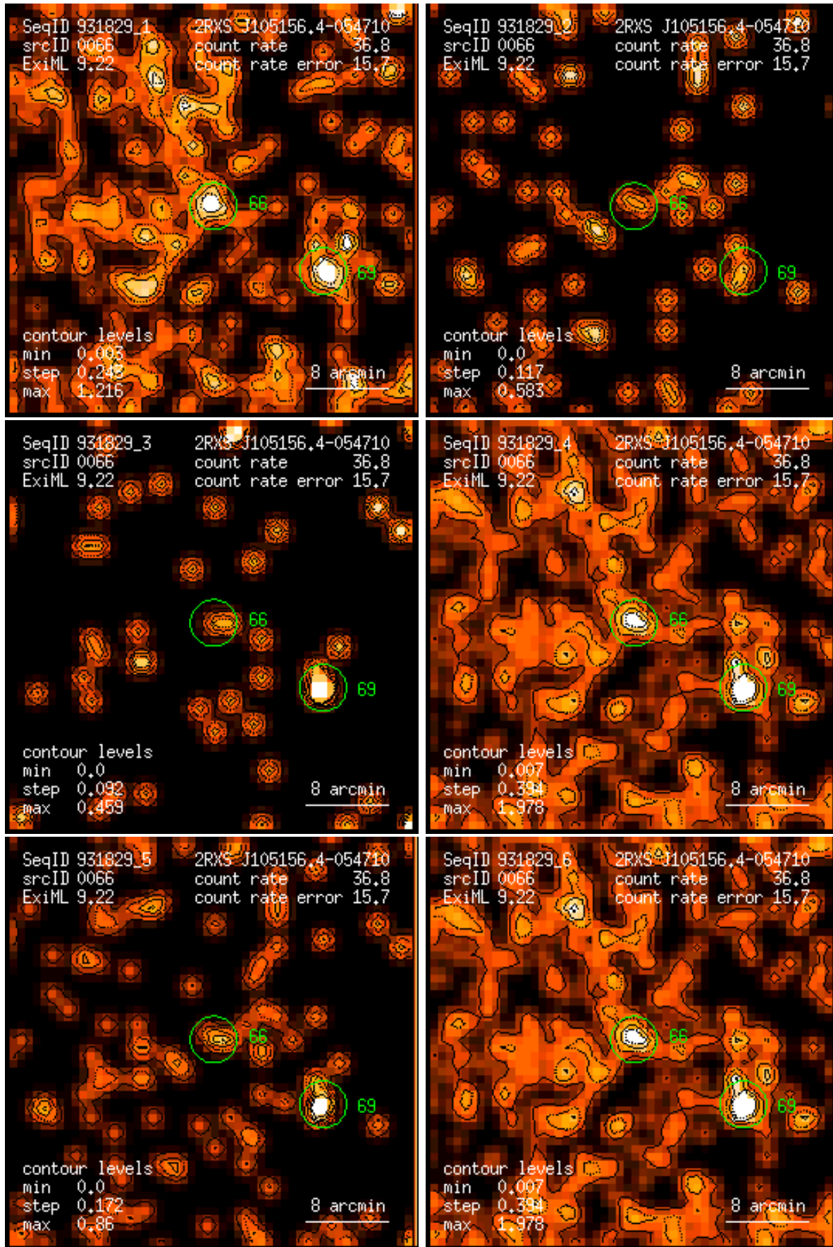
Figure 66: RASS 931829: detection 0066: band rate images, Gaussian filter: (1) PSPC channels 11 – 41, (2) 52 – 90, (3) 91 – 201, (4) 11 – 235, (5) 52 – 201, (6) 11 – 201. Broad band rates in counts/ks. Band rate contour levels in counts/ks/arcmin 2 .
