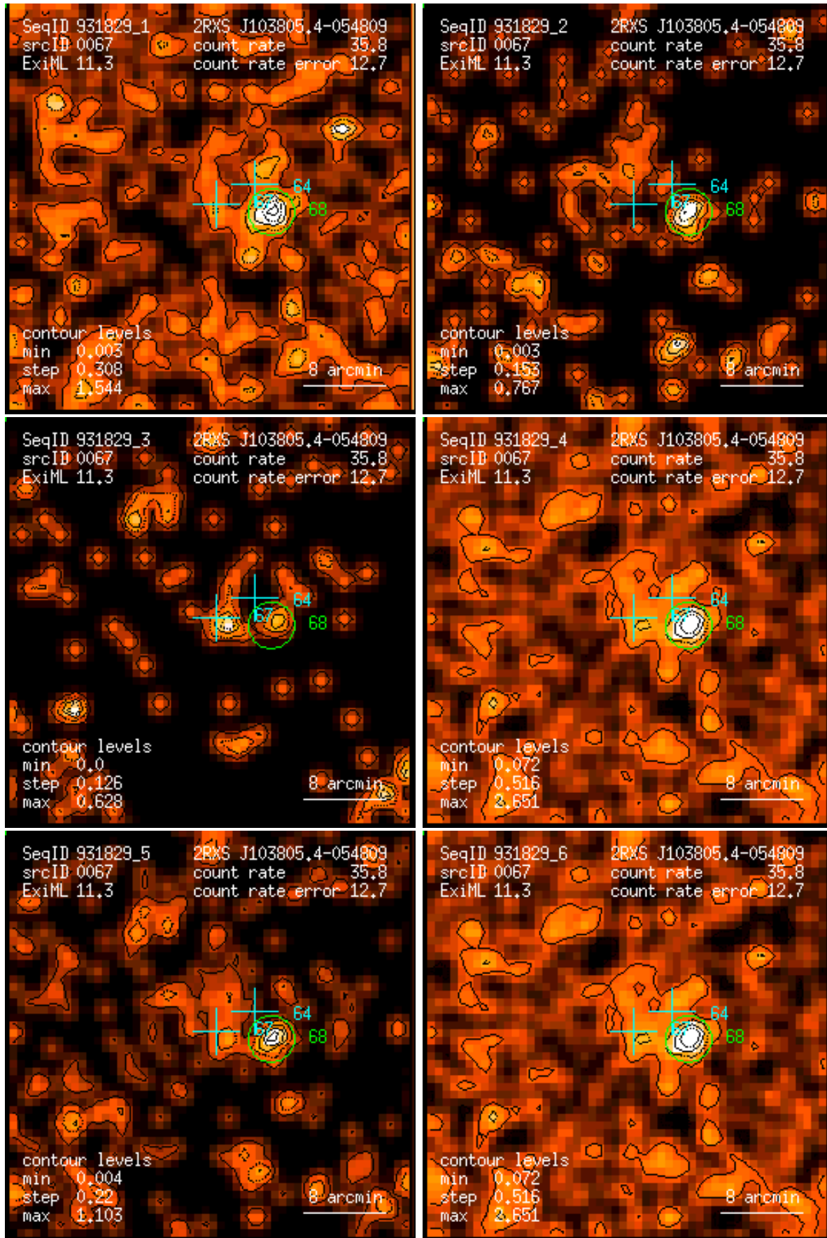
Figure 67: RASS 931829: detection 0067: band rate images, Gaussian filter: (1) PSPC channels 11 – 41, (2) 52 – 90, (3) 91 – 201, (4) 11 – 235, (5) 52 – 201, (6) 11 – 201. Broad band rates in counts/ks. Band rate contour levels in counts/ks/arcmin 2 .
