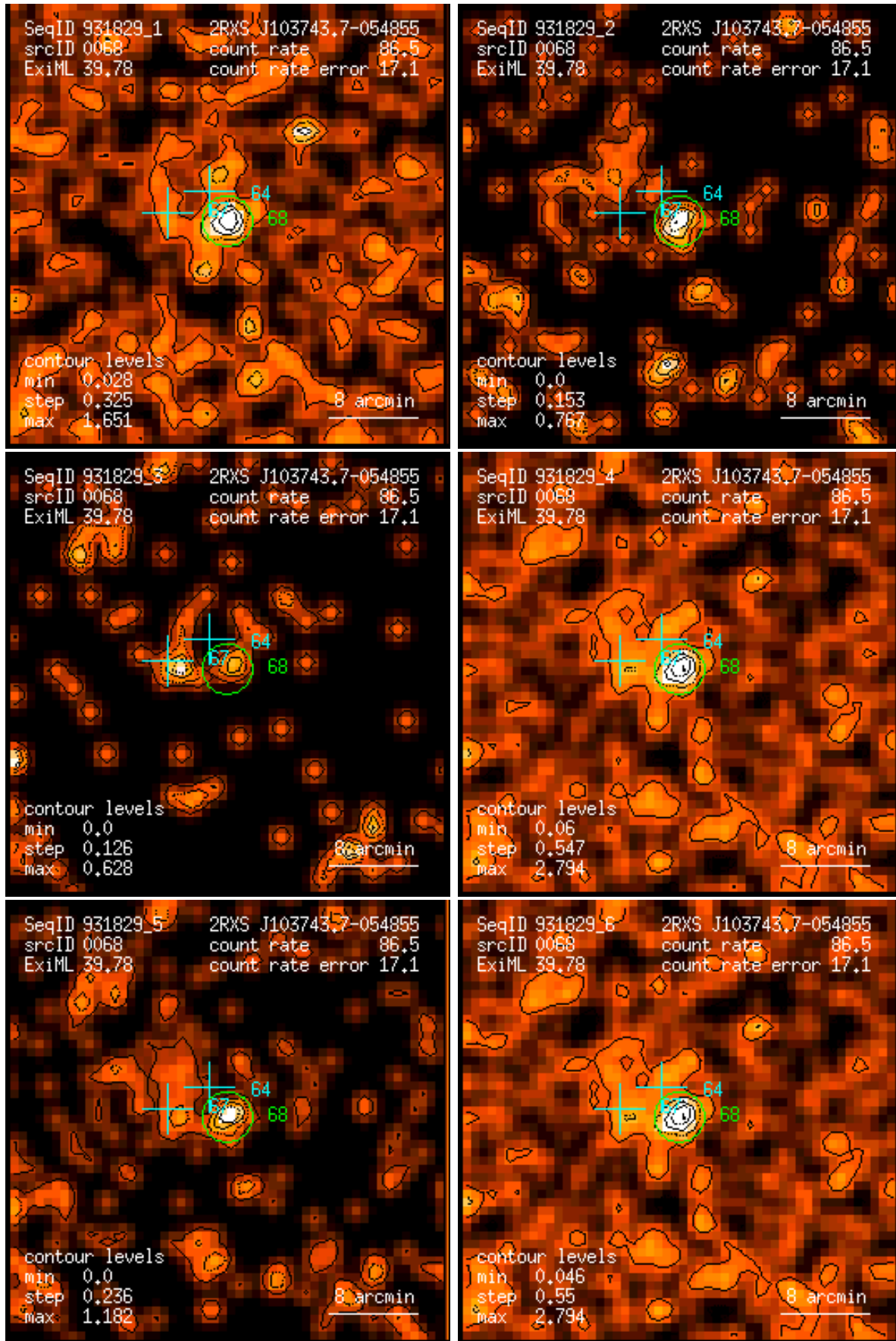
Figure 68: RASS 931829: detection 0068: band rate images, Gaussian filter: (1) PSPC channels 11 – 41, (2) 52 – 90, (3) 91 – 201, (4) 11 – 235, (5) 52 – 201, (6) 11 – 201. Broad band rates in counts/ks. Band rate contour levels in counts/ks/arcmin 2 .
