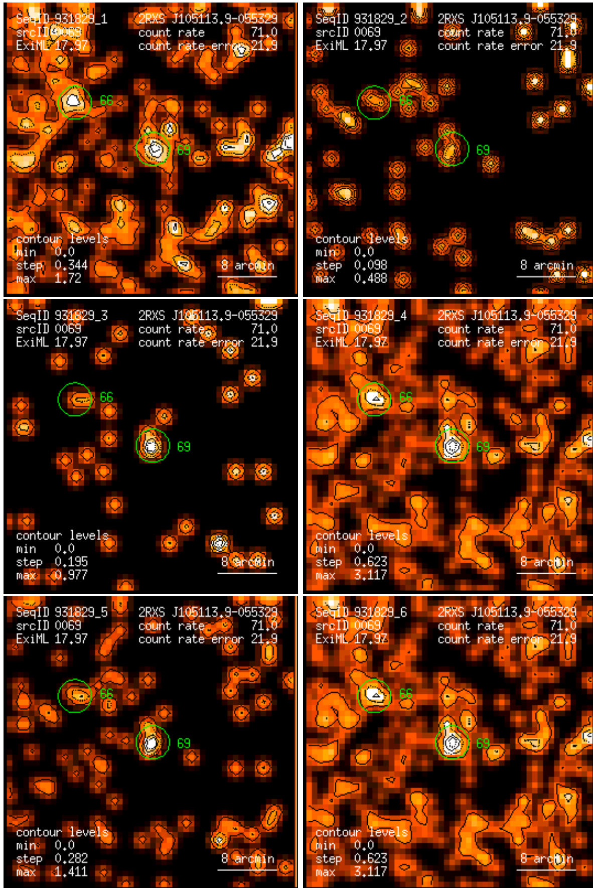
Figure 69: RASS 931829: detection 0069: band rate images, Gaussian filter: (1) PSPC channels 11 – 41, (2) 52 – 90, (3) 91 – 201, (4) 11 – 235, (5) 52 – 201, (6) 11 – 201. Broad band rates in counts/ks. Band rate contour levels in counts/ks/arcmin 2 .
