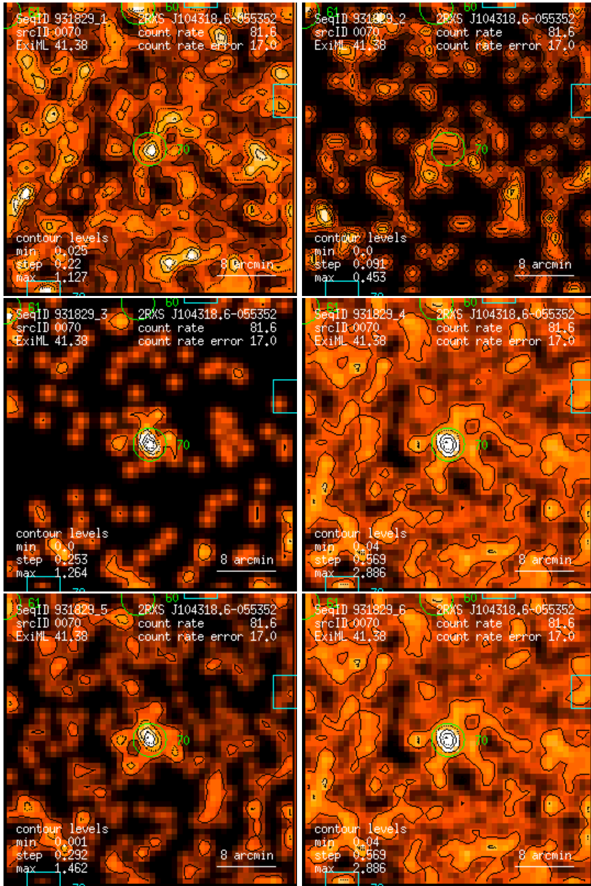
Figure 70: RASS 931829: detection 0070: band rate images, Gaussian filter: (1) PSPC channels 11 – 41, (2) 52 – 90, (3) 91 – 201, (4) 11 – 235, (5) 52 – 201, (6) 11 – 201. Broad band rates in counts/ks. Band rate contour levels in counts/ks/arcmin 2 .
