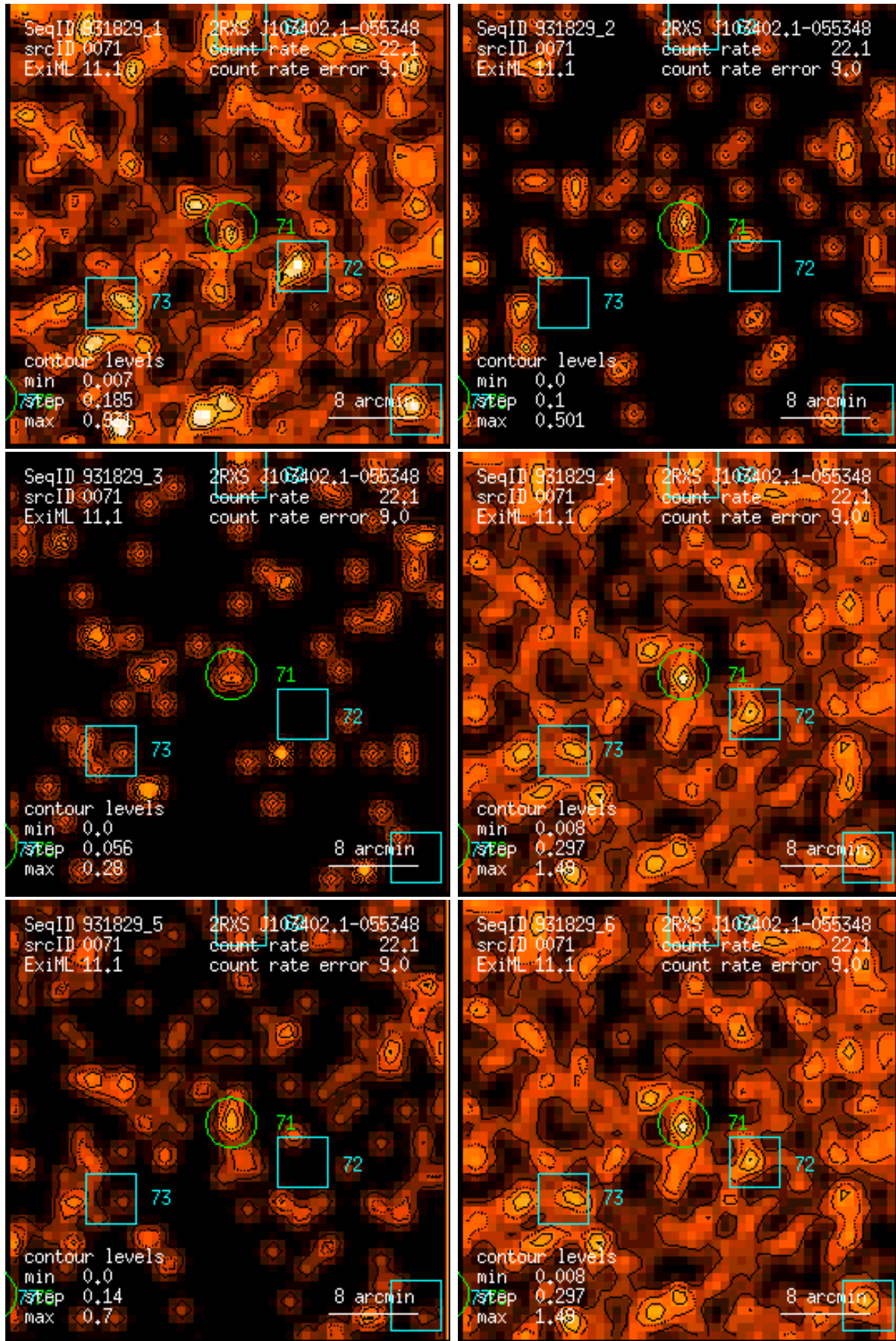
Figure 71: RASS 931829: detection 0071: band rate images, Gaussian filter: (1) PSPC channels 11 – 41, (2) 52 – 90, (3) 91 – 201, (4) 11 – 235, (5) 52 – 201, (6) 11 – 201. Broad band rates in counts/ks. Band rate contour levels in counts/ks/arcmin 2 .
