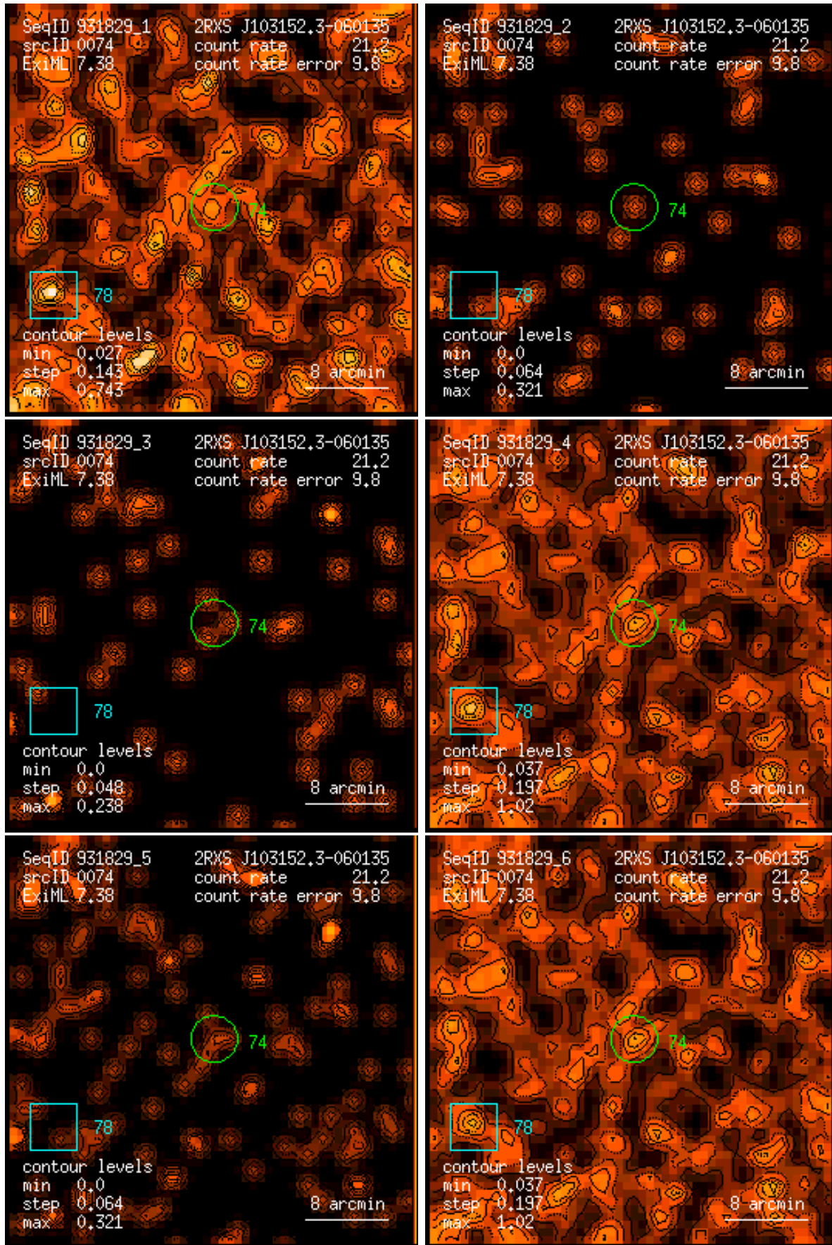
Figure 74: RASS 931829: detection 0074: band rate images, Gaussian filter: (1) PSPC channels 11 – 41, (2) 52 – 90, (3) 91 – 201, (4) 11 – 235, (5) 52 – 201, (6) 11 – 201. Broad band rates in counts/ks. Band rate contour levels in counts/ks/arcmin 2 .
