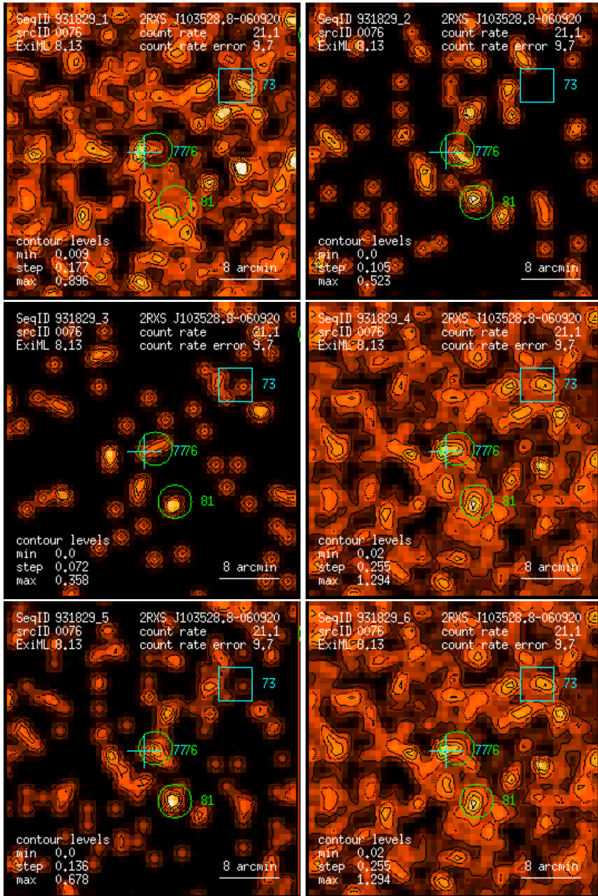
Figure 76: RASS 931829: detection 0076: band rate images, Gaussian filter: (1) PSPC channels 11 – 41, (2) 52 – 90, (3) 91 – 201, (4) 11 – 235, (5) 52 – 201, (6) 11 – 201. Broad band rates in counts/ks. Band rate contour levels in counts/ks/arcmin 2 .
