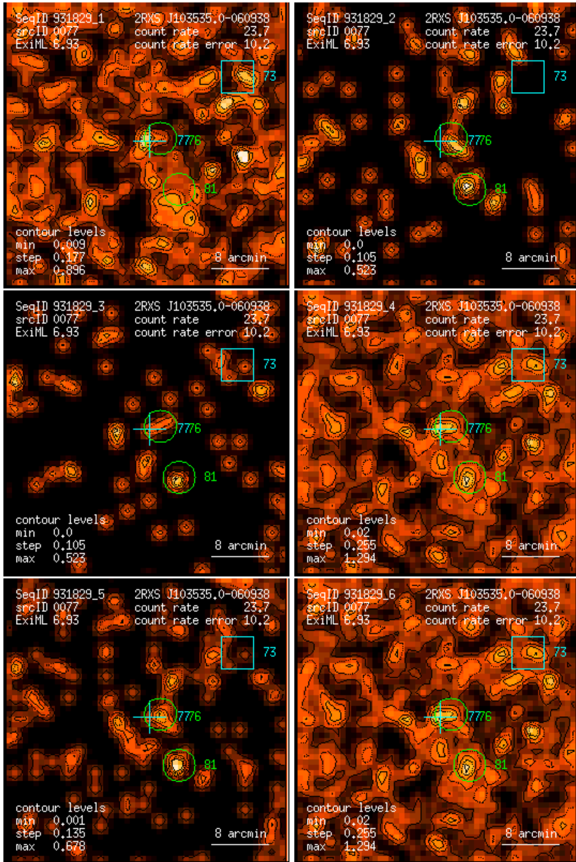
Figure 77: RASS 931829: detection 0077: band rate images, Gaussian filter: (1) PSPC channels 11 – 41, (2) 52 – 90, (3) 91 – 201, (4) 11 – 235, (5) 52 – 201, (6) 11 – 201. Broad band rates in counts/ks. Band rate contour levels in counts/ks/arcmin 2 .
