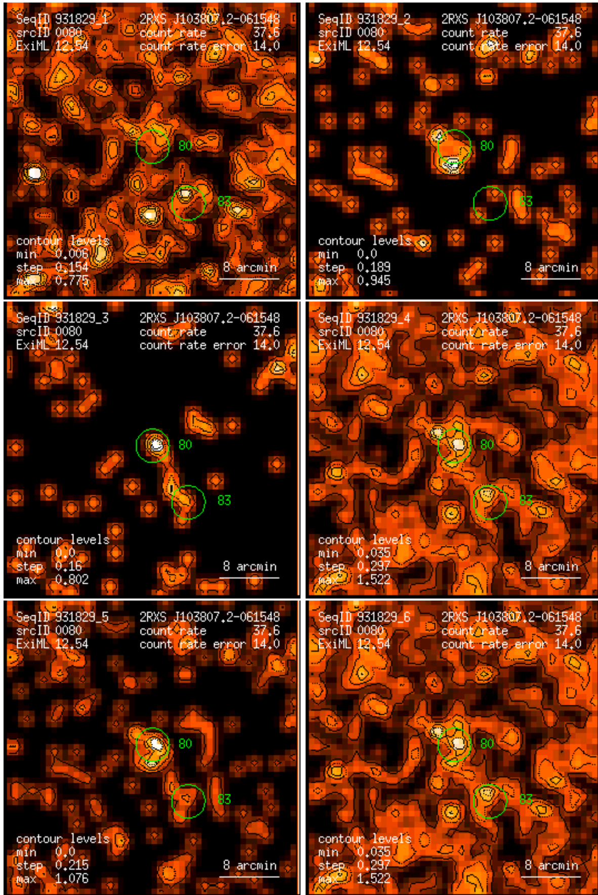
Figure 80: RASS 931829: detection 0080: band rate images, Gaussian filter: (1) PSPC channels 11 – 41, (2) 52 – 90, (3) 91 – 201, (4) 11 – 235, (5) 52 – 201, (6) 11 – 201. Broad band rates in counts/ks. Band rate contour levels in counts/ks/arcmin 2 .
