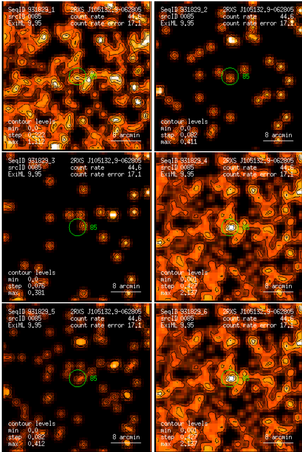
Figure 85: RASS 931829: detection 0085: band rate images, Gaussian filter: (1) PSPC channels 11 – 41, (2) 52 – 90, (3) 91 – 201, (4) 11 – 235, (5) 52 – 201, (6) 11 – 201. Broad band rates in counts/ks. Band rate contour levels in counts/ks/arcmin 2 .
