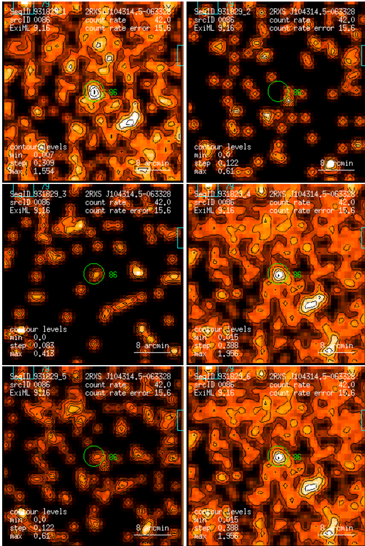
Figure 86: RASS 931829: detection 0086: band rate images, Gaussian filter: (1) PSPC channels 11 – 41, (2) 52 – 90, (3) 91 – 201, (4) 11 – 235, (5) 52 – 201, (6) 11 – 201. Broad band rates in counts/ks. Band rate contour levels in counts/ks/arcmin 2 .
