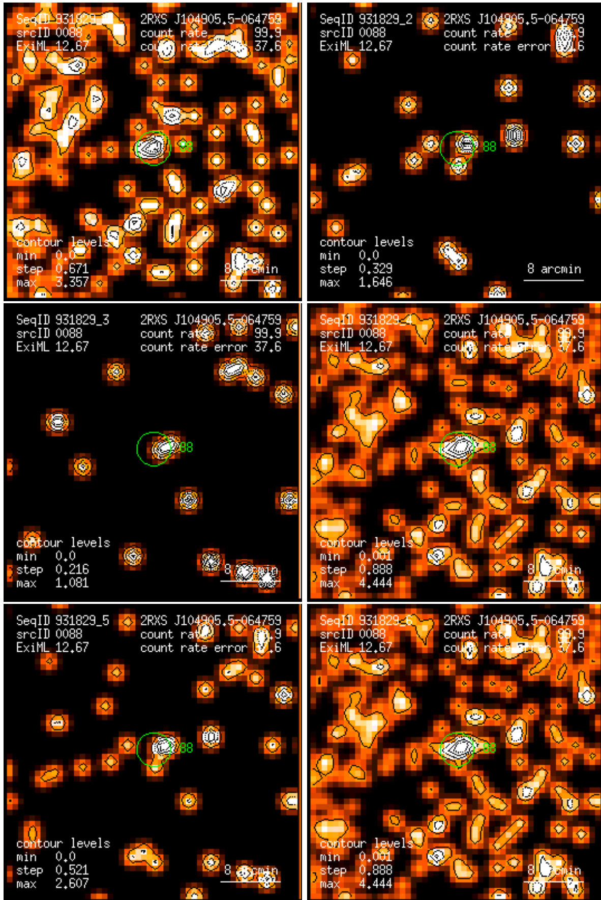
Figure 88: RASS 931829: detection 0088: band rate images, Gaussian filter: (1) PSPC channels 11 – 41, (2) 52 – 90, (3) 91 – 201, (4) 11 – 235, (5) 52 – 201, (6) 11 – 201. Broad band rates in counts/ks. Band rate contour levels in counts/ks/arcmin 2 .
