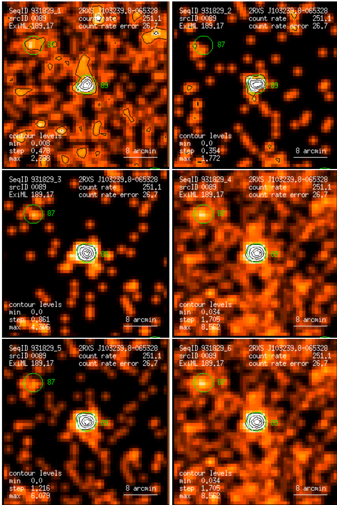
Figure 89: RASS 931829: detection 0089: band rate images, Gaussian filter: (1) PSPC channels 11 – 41, (2) 52 – 90, (3) 91 – 201, (4) 11 – 235, (5) 52 – 201, (6) 11 – 201. Broad band rates in counts/ks. Band rate contour levels in counts/ks/arcmin 2 .
