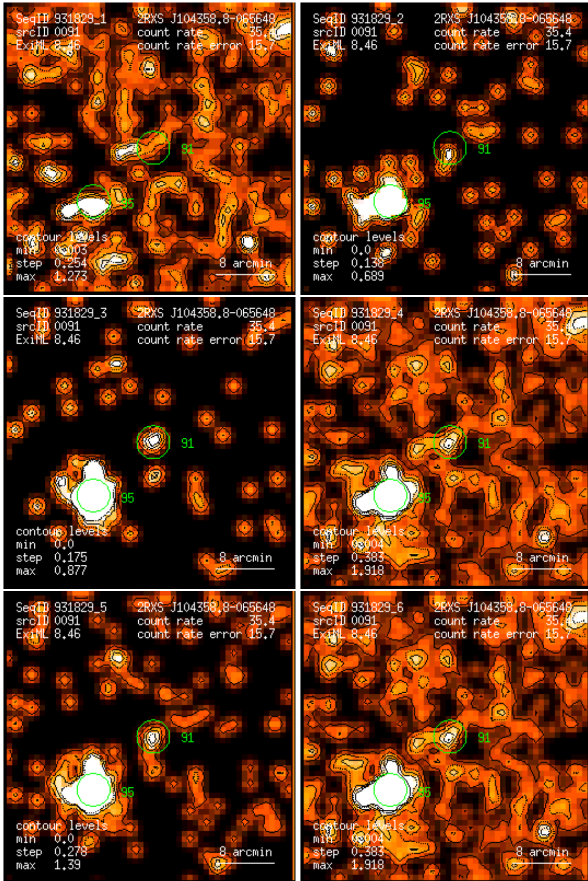
Figure 91: RASS 931829: detection 0091: band rate images, Gaussian filter: (1) PSPC channels 11 – 41, (2) 52 – 90, (3) 91 – 201, (4) 11 – 235, (5) 52 – 201, (6) 11 – 201. Broad band rates in counts/ks. Band rate contour levels in counts/ks/arcmin 2 .
