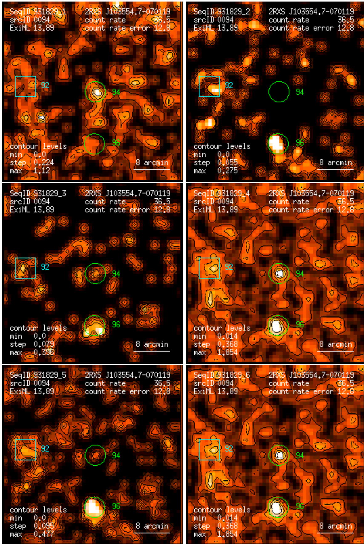
Figure 94: RASS 931829: detection 0094: band rate images, Gaussian filter: (1) PSPC channels 11 – 41, (2) 52 – 90, (3) 91 – 201, (4) 11 – 235, (5) 52 – 201, (6) 11 – 201. Broad band rates in counts/ks. Band rate contour levels in counts/ks/arcmin 2 .
