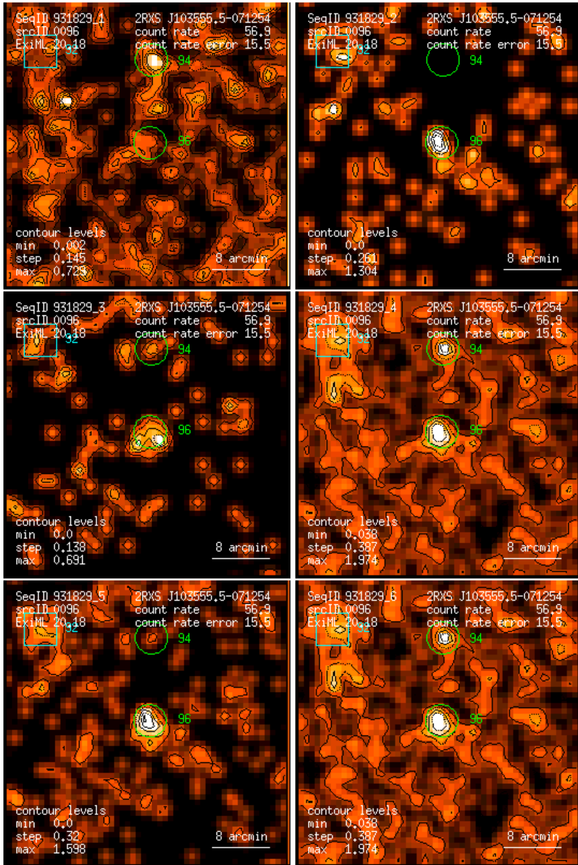
Figure 96: RASS 931829: detection 0096: band rate images, Gaussian filter: (1) PSPC channels 11 – 41, (2) 52 – 90, (3) 91 – 201, (4) 11 – 235, (5) 52 – 201, (6) 11 – 201. Broad band rates in counts/ks. Band rate contour levels in counts/ks/arcmin 2 .
