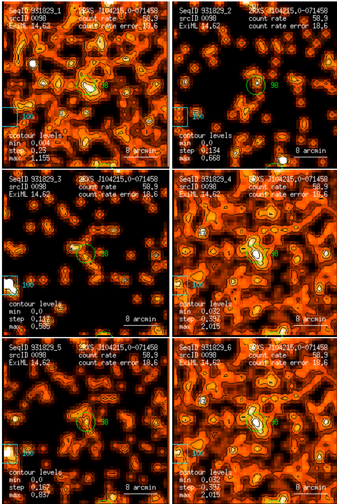
Figure 98: RASS 931829: detection 0098: band rate images, Gaussian filter: (1) PSPC channels 11 – 41, (2) 52 – 90, (3) 91 – 201, (4) 11 – 235, (5) 52 – 201, (6) 11 – 201. Broad band rates in counts/ks. Band rate contour levels in counts/ks/arcmin 2 .
