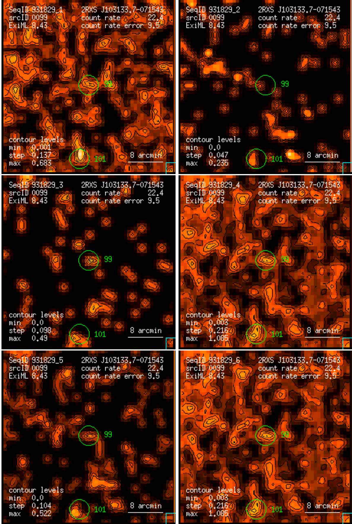
Figure 99: RASS 931829: detection 0099: band rate images, Gaussian filter: (1) PSPC channels 11 – 41, (2) 52 – 90, (3) 91 – 201, (4) 11 – 235, (5) 52 – 201, (6) 11 – 201. Broad band rates in counts/ks. Band rate contour levels in counts/ks/arcmin 2 .
