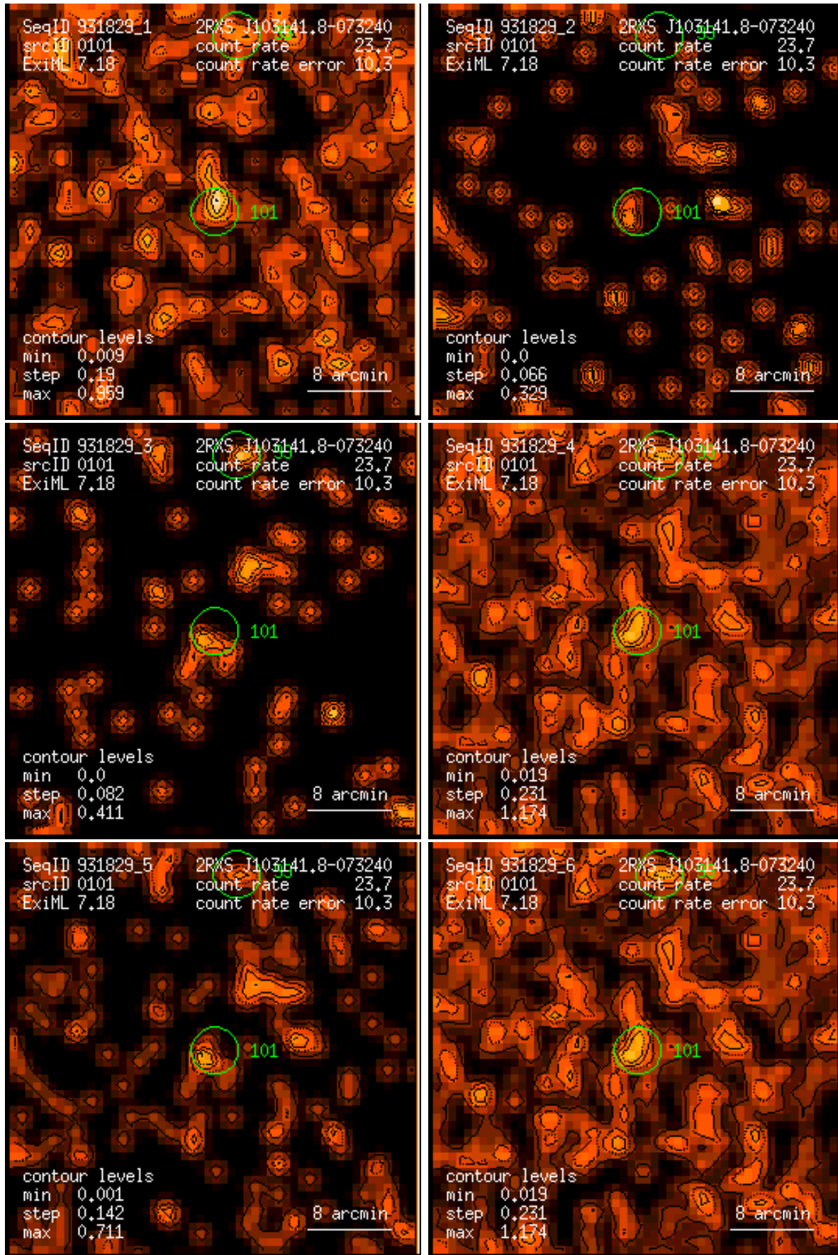
Figure 101: RASS 931829: detection 0101: band rate images, Gaussian filter: (1) PSPC channels 11 – 41, (2) 52 – 90, (3) 91 – 201, (4) 11 – 235, (5) 52 – 201, (6) 11 – 201. Broad band rates in counts/ks. Band rate contour levels in counts/ks/arcmin 2 .
