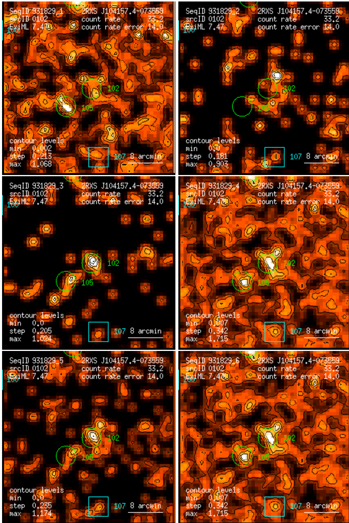
Figure 102: RASS 931829: detection 0102: band rate images, Gaussian filter: (1) PSPC channels 11 – 41, (2) 52 – 90, (3) 91 – 201, (4) 11 – 235, (5) 52 – 201, (6) 11 – 201. Broad band rates in counts/ks. Band rate contour levels in counts/ks/arcmin 2 .
