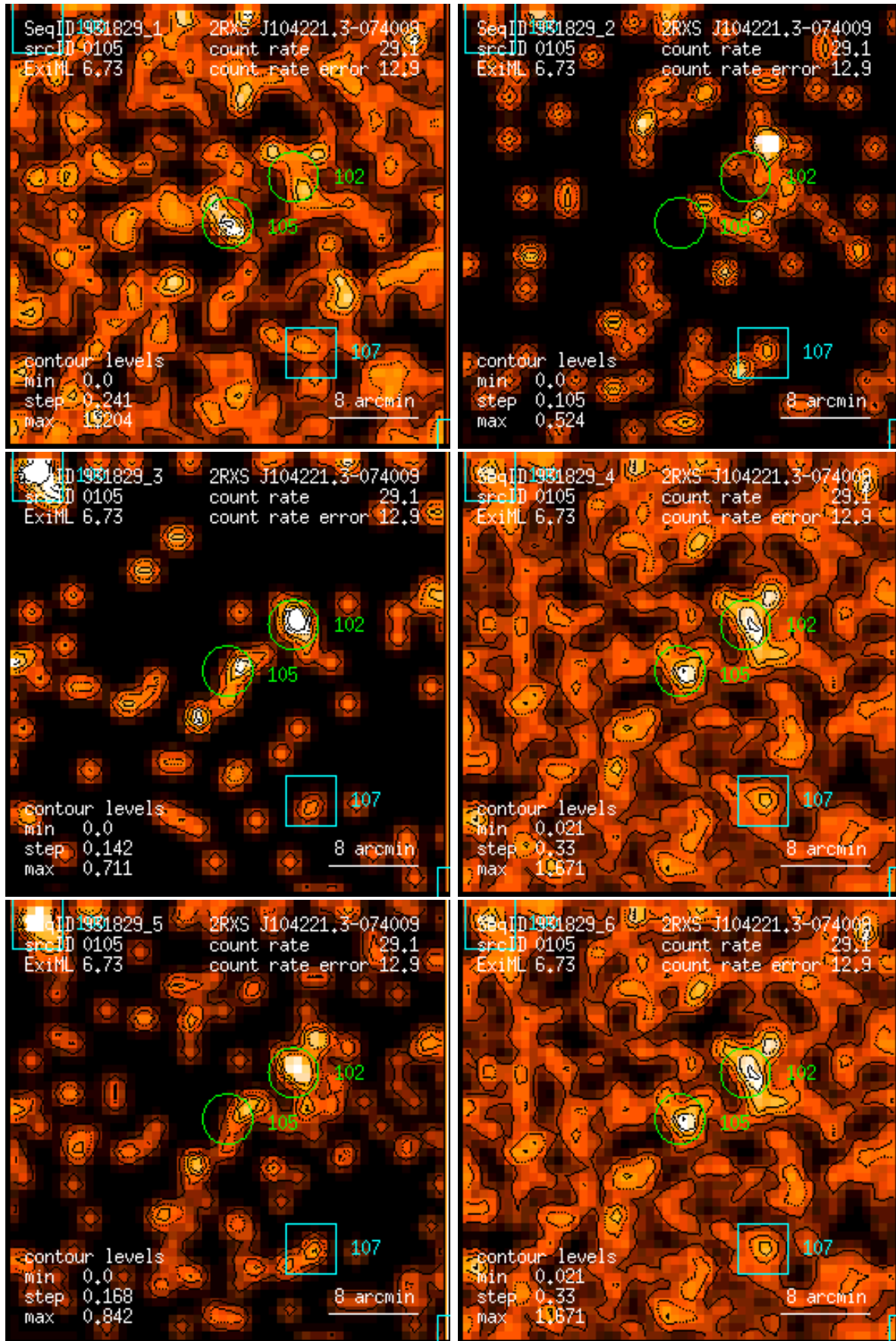
Figure 105: RASS 931829: detection 0105: band rate images, Gaussian filter: (1) PSPC channels 11 – 41, (2) 52 – 90, (3) 91 – 201, (4) 11 – 235, (5) 52 – 201, (6) 11 – 201. Broad band rates in counts/ks. Band rate contour levels in counts/ks/arcmin 2 .
