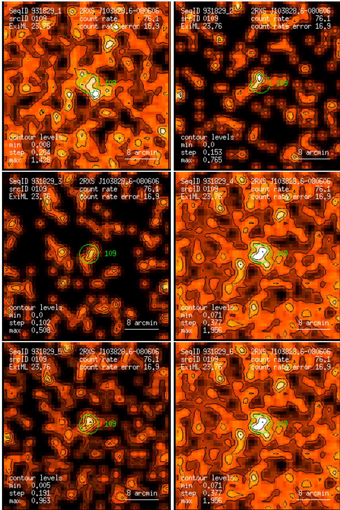
Figure 109: RASS 931829: detection 0109: band rate images, Gaussian filter: (1) PSPC channels 11 – 41, (2) 52 – 90, (3) 91 – 201, (4) 11 – 235, (5) 52 – 201, (6) 11 – 201. Broad band rates in counts/ks. Band rate contour levels in counts/ks/arcmin 2 .
